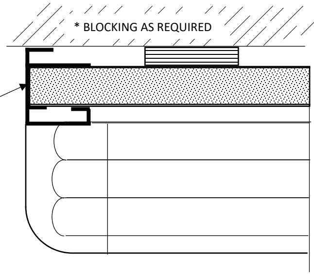
TOP SECTION VIEW
